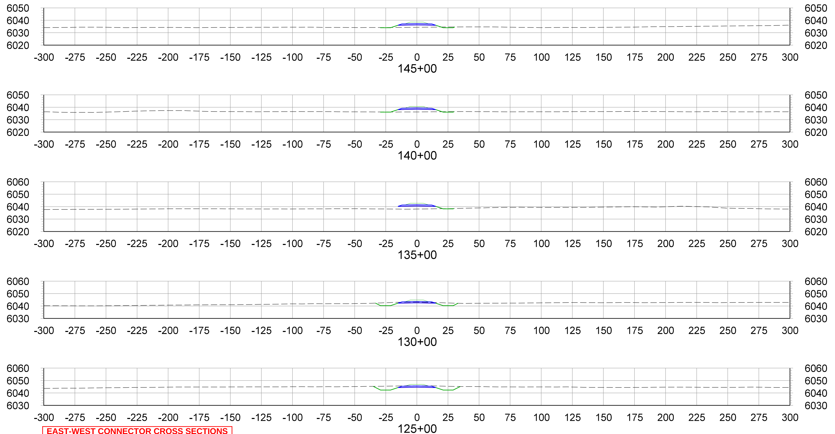
CROSS SECTIONS STA.125+00 TO STA.145+00
