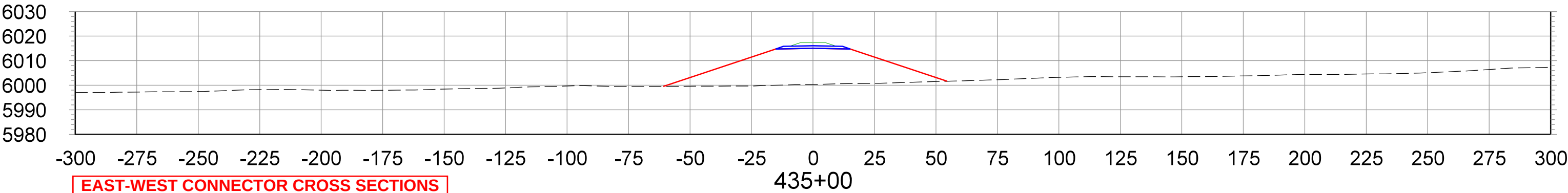
CROSS SECTIONS STA.435+00 TO STA.450+00
