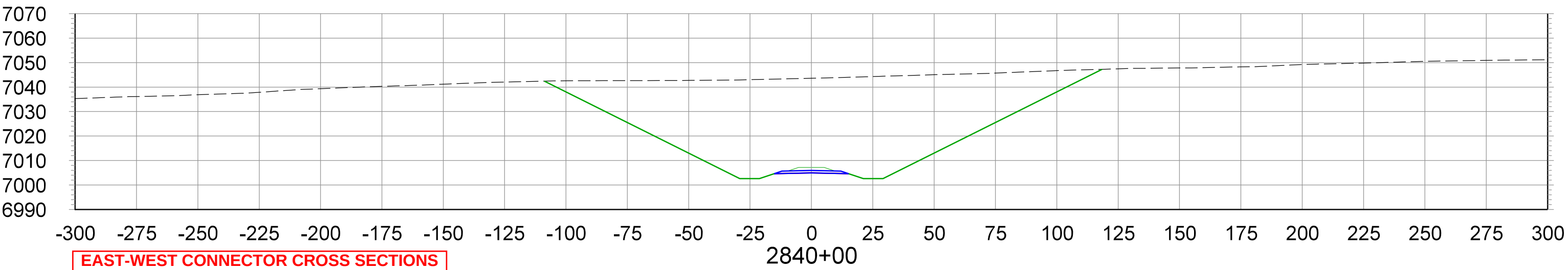
CROSS SECTIONS STA.2840+00 TO STA.2855+00
