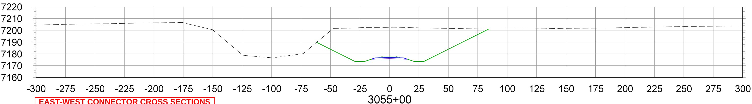
CROSS SECTIONS STA.3055+00 TO STA.3068+96
