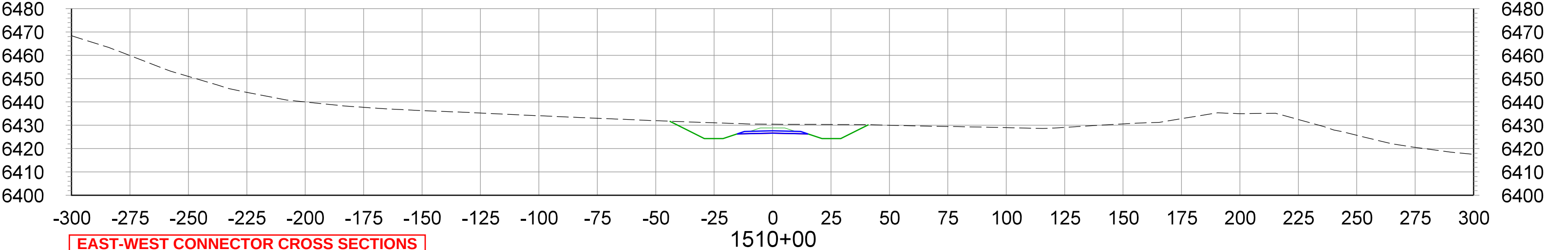
CROSS SECTIONS STA.1510+00 TO STA.1525+00
