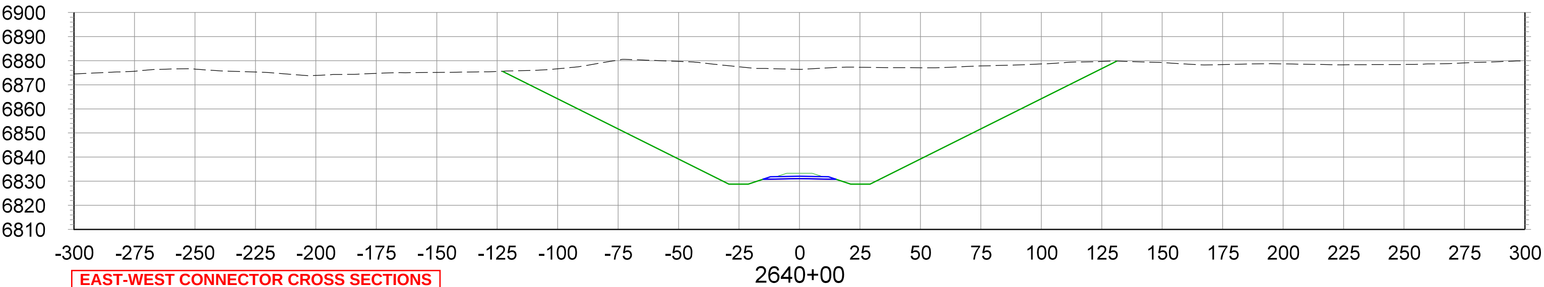
CROSS SECTIONS STA.2640+00 TO STA.2655+00
