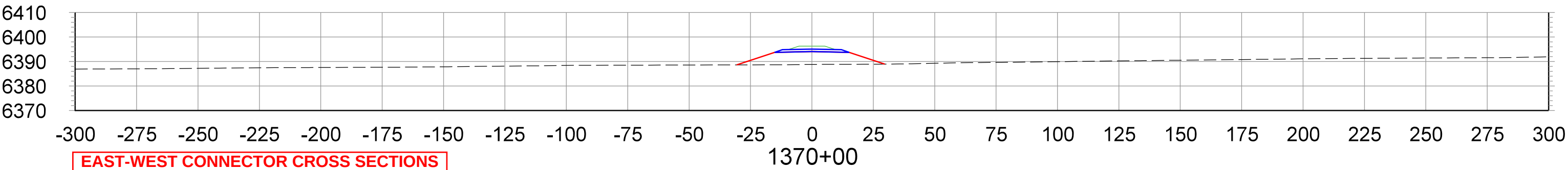
CROSS SECTIONS STA.1370+00 TO STA.1385+00
