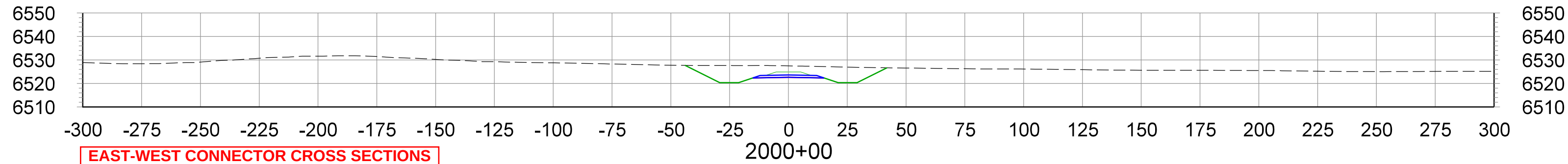
CROSS SECTIONS STA.2000+00 TO STA.2020+00
